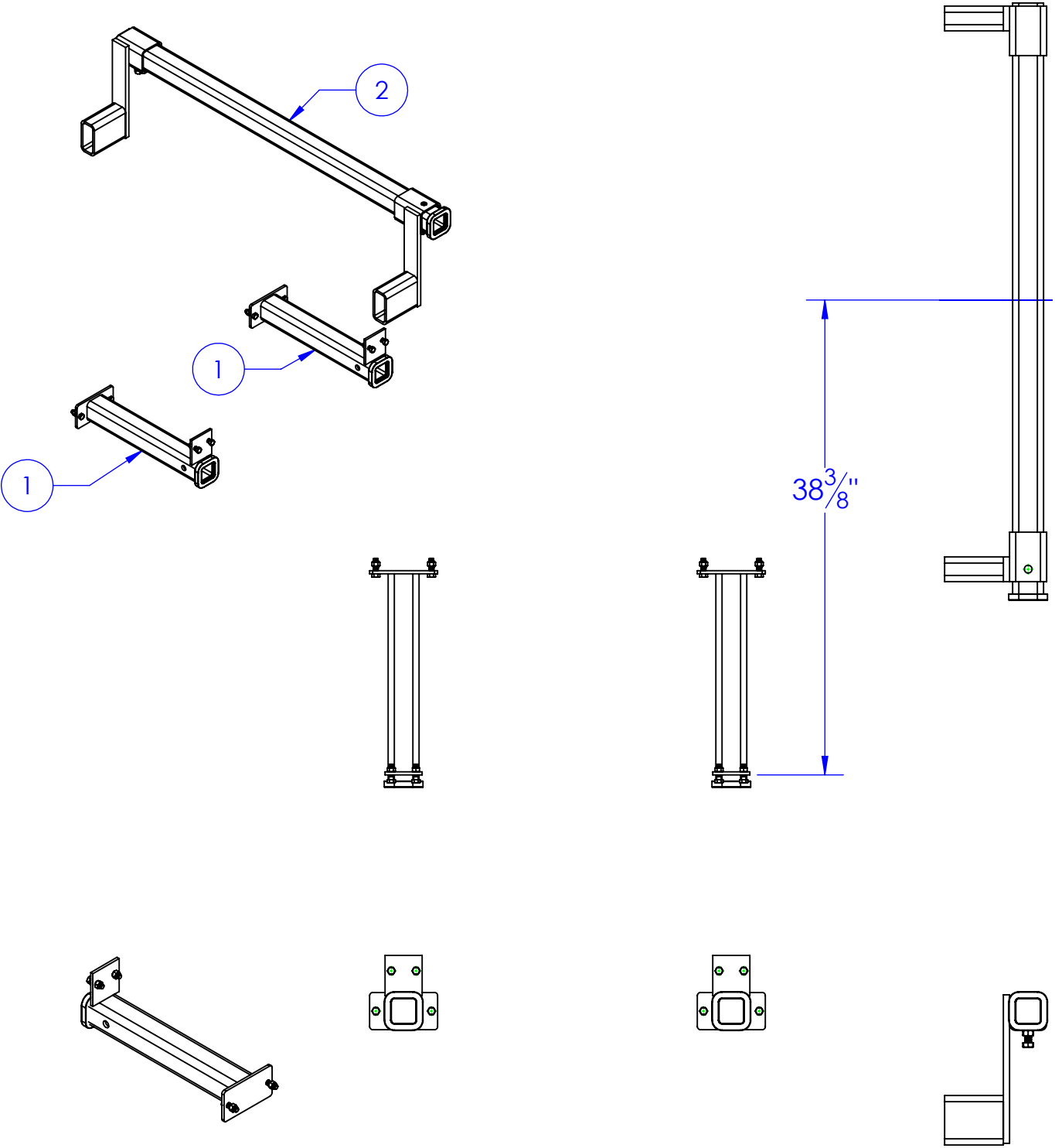
OP-PIPE H-PS100 REAR HOLDER
